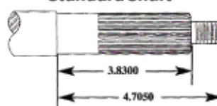
Standard Shaft
